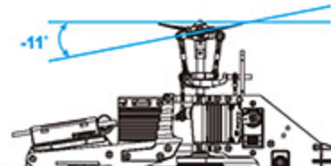
Stick Position at Low/Throttle 100%/Pitch -11° 搖桿低速/油門100%/Pitch -11°
