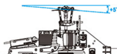
Stick Position at Hovering/Throttle 65%~70%/Pitch +5° 搖桿停懸/油門65%~70%/Pitch +5°
